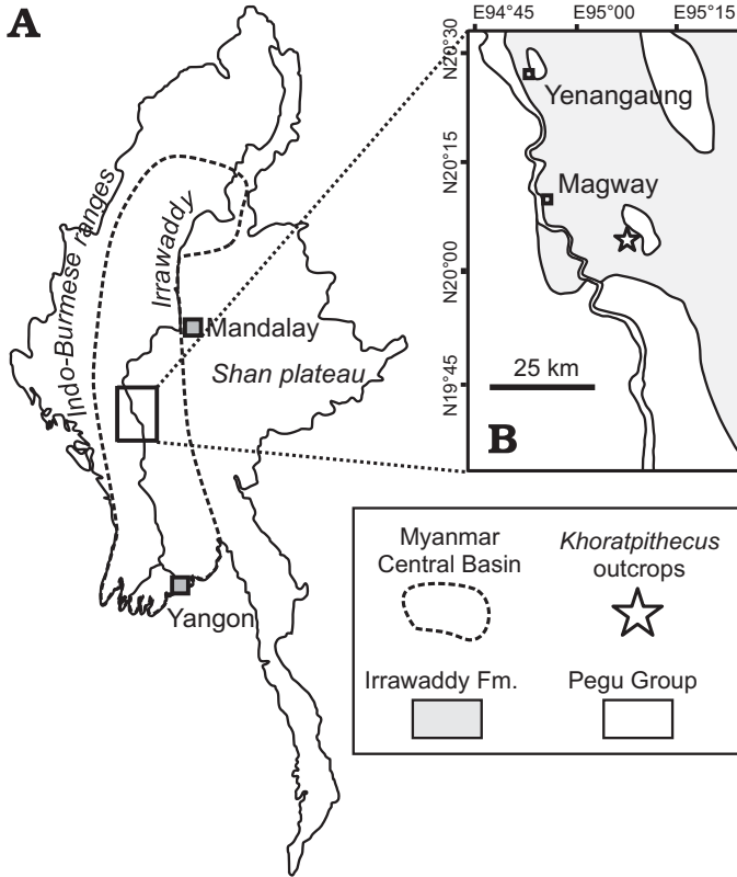
Fig. 1. A. Map of Myanmar showing the area of study within the Myanmar Central Basin. B. Detailed map of the Magway region positioning the outcrops that yielded the chalicothere mandible MFI-105.
