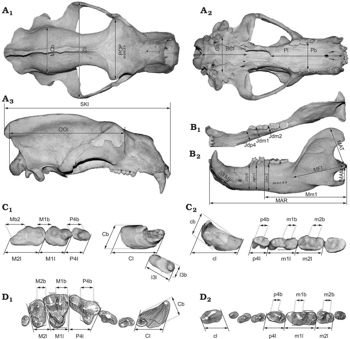
Fig. 1. Osteological measurements used in the regression analyses for the craniodental skeleton, illustrated on a skull of Ursus maritimus . A. Cranium in dorsal (A 1 ), ventral (A 2 ) and lateral (A 3 ) views. B. Mandible in occlusal (B 1 ) and lateral (B 2 ) views. C. Upper (C 1 ) and lower (C 2 ) dentition. D. Daphoenodon falkenbachi , upper (D 1 ) and lower (D 2 ) dentition (modified from Hunt 2002; upper teeth reversed). For abbreviations and definitions of measurements, see Table 2.
