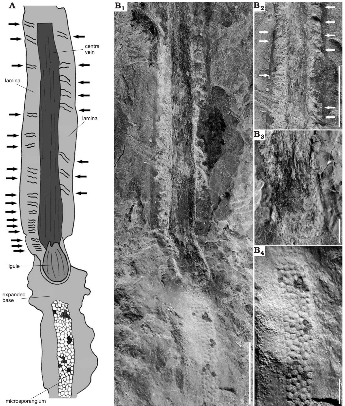
Fig. 2. Isoetean microsporophyll with in situ masses of microspores, from the Boundary Marls unit (uppermost Albian) of Estercuel (Teruel, Spain). A. Explanatory drawing of the microsporophyll in B. Black arrows and the irregular lines indicate the impressions of trabeculae in leaf section. B. MPZ 2010/919. Microsporophyll with the sporangium at base containing masses of microspores ( B 1 ). Detail of the microsporophyll lamina with impressions of trabeculae indicated by white arrows ( B 2 ). Detail of the base of the microsporophyll leaf showing the impression of ligule ( B 3 ). Microsporangium containing masses of microspores ( B 4 ). Scale bars: A, B 1 , B 2 , 5 mm; B 3 , B 4 , 1 mm.
