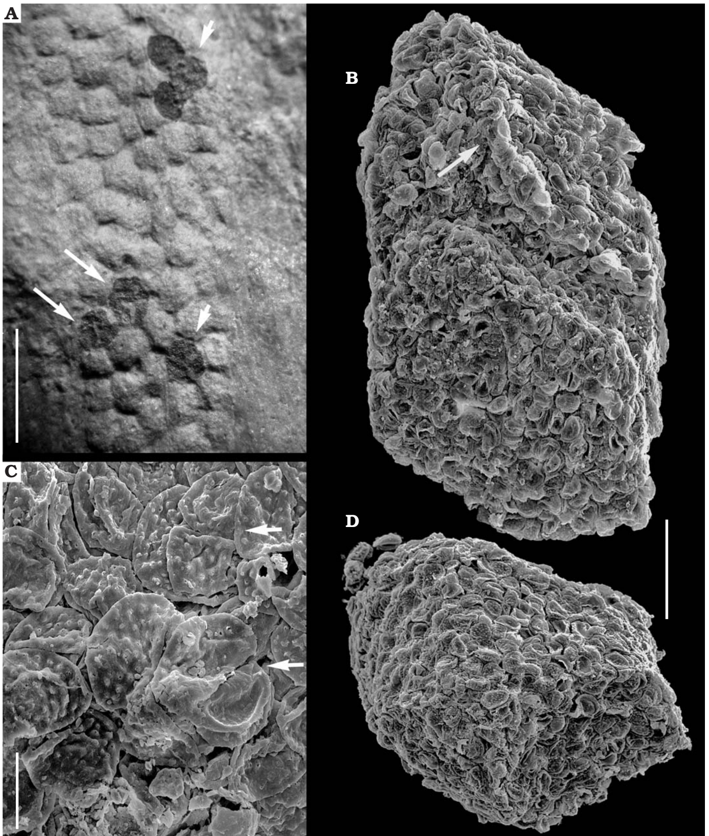
Fig. 3. In situ masses of microspores of isoetalean microsporophyll (MPZ 2010/919) from Estercuel locality, latest Albian. A. Detail of the microsporangium with six masses of microspores, some of them showing a false "trilete" mark (arrows) probably due to a post-sedimentary compression process. B, D. Masses of hundreds of microspores, the false "trilete" mark due to compaction within adjacent polygonal bodies inside microsporophyll (arrow). C. Detail of microspores presumably grouped in tetrads (arrows) showing both proximal and distal faces. B–D, SEM micrographs. Scale bars: A, 5 mm; B, D, 100 \mu m; C, 20 \mu m.
