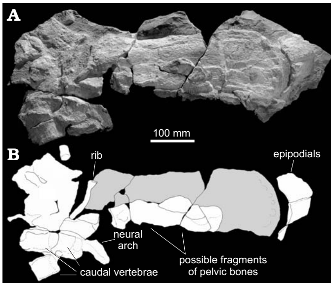
Fig. 6. Caudal vertebrae and hindlimb elements of the unidentified pliosaurid (MPPL 18797) from the uppermost Callovian–middle Oxfordian of Kaberlaba (Asiago, Italy). Photograph (A) and explanatory drawing (B). Grey tones indicate the femur.
