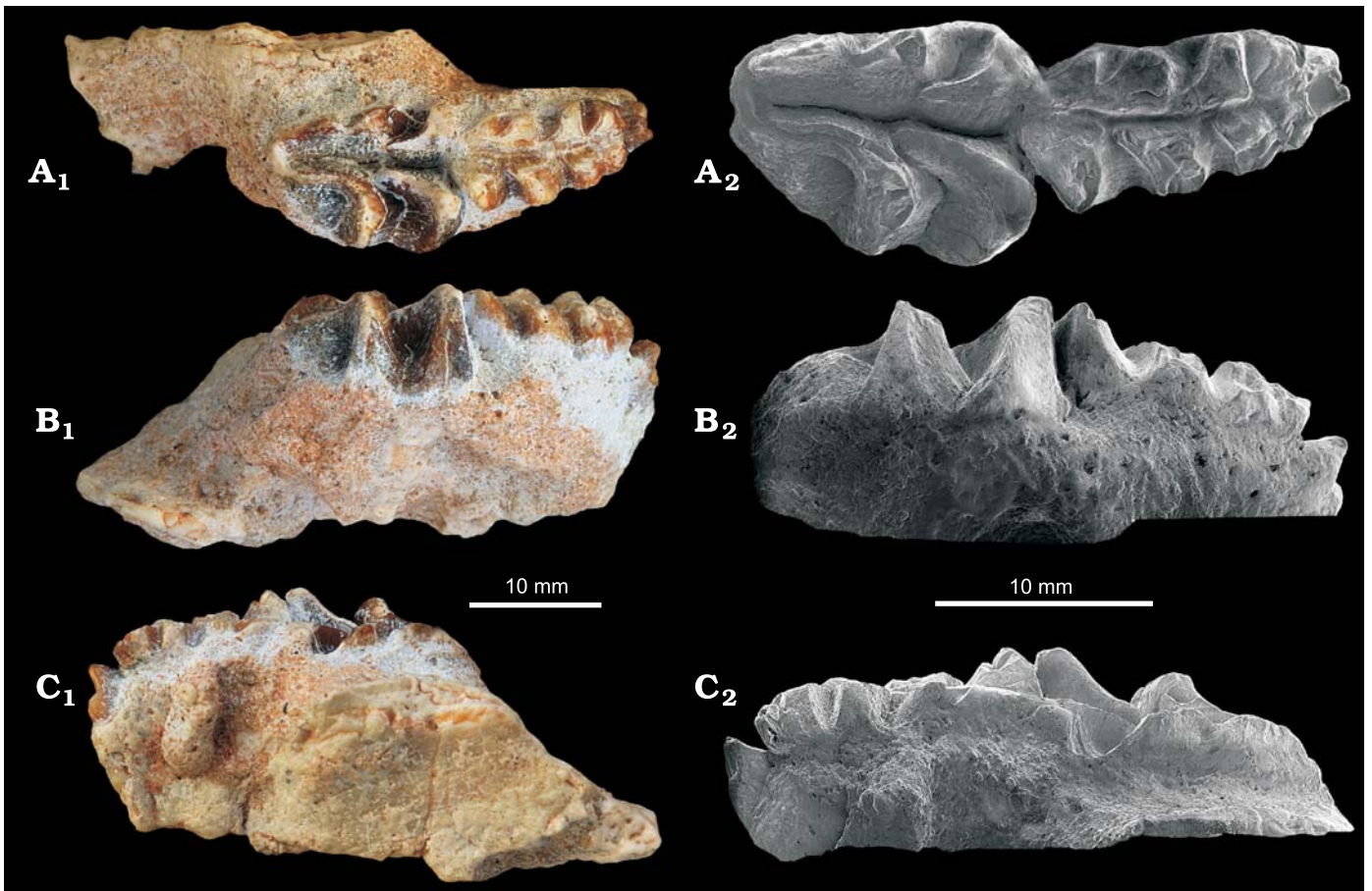
Fig. 7. Multituberculate mammal Sphenopsalis nobilis Matthew, Granger, and Simpson, 1928 (IVPP V19032) from the upper Paleocene Nomogen beds at the Erden (Urtyn) Obo locality, Inner Mongolia, China. Left lower cheek teeth (p4–m2) from the same individual as in Fig. 5 in occlusal (A), medial (B), and lateral (C) views. Photographs (A 1 –C 1 ), SEM images (A 2 –C 2 ).
