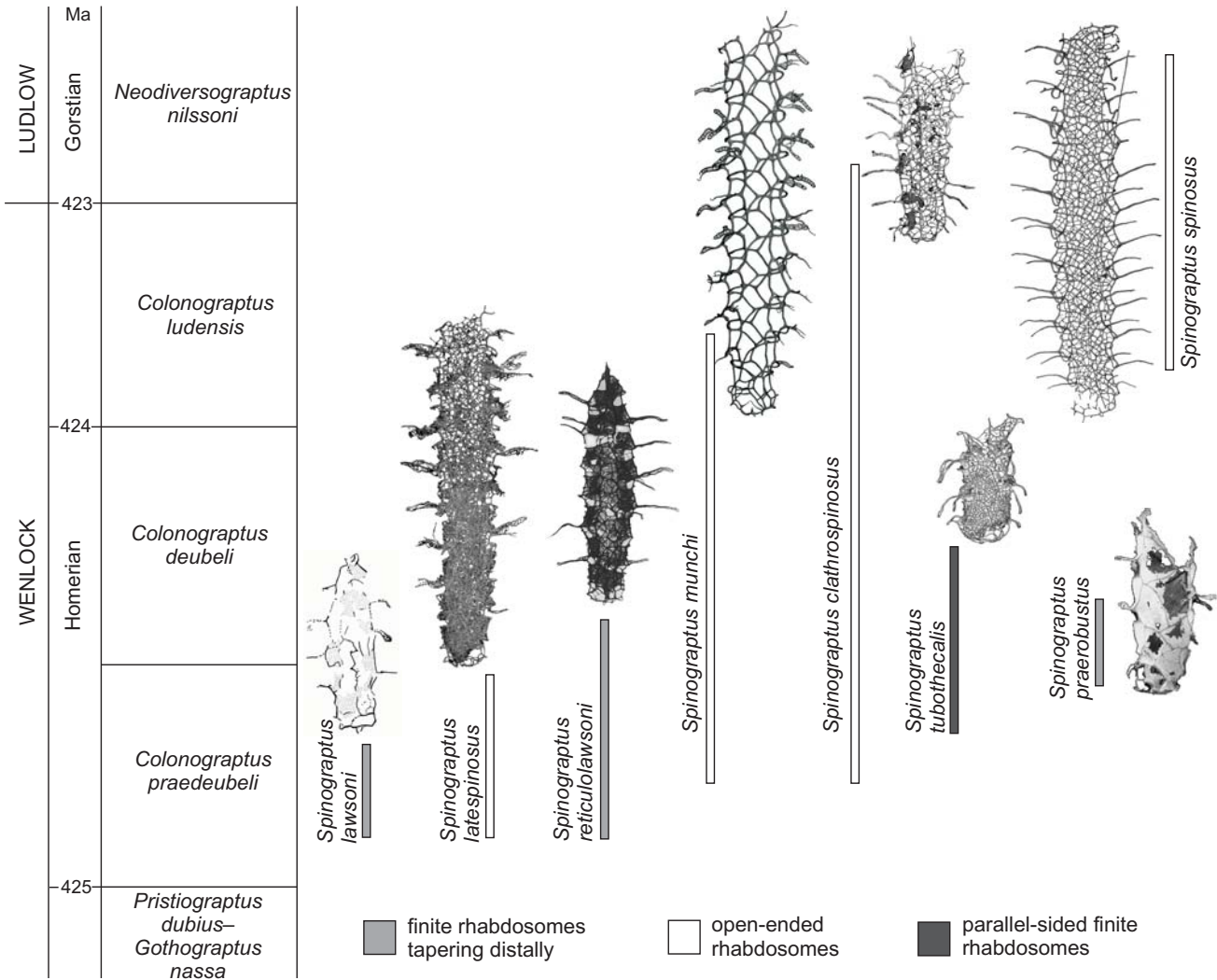
Fig. 1. Stratigraphical sequence of the Spinograptus species, with new data from this paper and Kozłowska-Dawidziuk 1997: fig. 12. The ranges of Spinograptus spinosus (Wood, 1900) and S. clathrospinosus Eisenack, 1951 reach the Saetograptus linearis – Monograptus ceratus Biozone in the Arctic Canada (Lenz and Kozłowska-Dawidziuk 2004), which is not marked herein.
