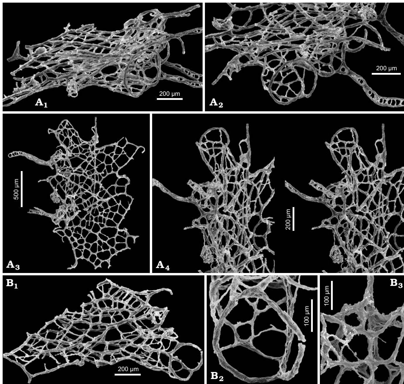
Fig. 4. Retiolitid graptolite Spinograptus tubothecalis sp. nov. from Prągowiec 2, Colonograptus deubeli Biozone. A. ZPAL G. 47/6, paratype, distal end of rhabdosome with three well preserved thecae on one side and small appendix; distal view ( A_1 ), view towards the inside of last theca ( A_2 ), lateral view of whole specimen ( A_3 ), stereopair of the better preserved thecae ( A_4 ). B. ZPAL G. 47/7, distal end of rhabdosome with two last thecae and terminal structure; distal view of the whole fragment ( B_1 ); view to the inside of last theca ( B_2 ); terminal structure ( B_3 ).
