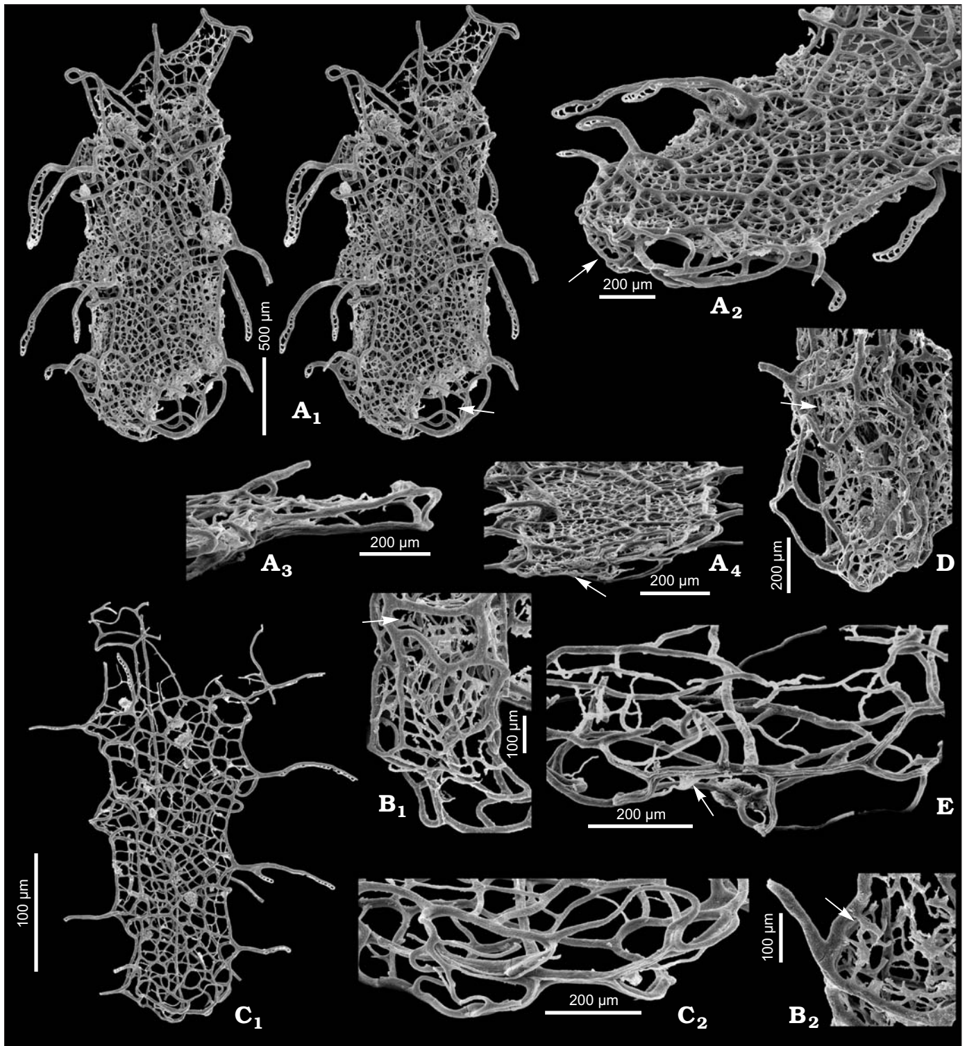
Fig. 2. Retiolitid graptolites Spinograptus tubothecalis sp. nov. and Spinograptus clathrospinosus Eisenack, 1951 from the Gołdap IG-1 borehole, Poland. A, B, D, E. Spinograptus tubothecalis sp. nov., depth 1267.0 m, Colonograptus deubeli Biozone, Wenlock. A. ZPAL G. 47/1, holotype, stereopair of obverse view of finite rhabdosome, proximal lateral orifice (arrow) ( A 1 ); proximal view of rhabdosome ( A 2 ), outer ancora arrowed; proximal view of isolated last theca and nema ( A 3 ); ancora umbrella and dense outer ancora at th 1 1 side of rhabdosome (arrow) ( A 4 ). B. ZPAL G. 47/5, th 1 1 side view of proximal part of rhabdosome showing dense outer ancora and pre-thecal ventral orifice overgrown by reticulum (arrow) ( B 1 ), rudimentary transverse rod (arrow) ( B 2 ). D. ZPAL G. 47/8, th 1 2 side view of proximal part of rhabdosome showing overgrown pre-thecal ventral orifice (arrow). E. ZPAL G. 47/9, proximal view of immature rhabdosome showing ancora umbrella and outer ancora starting to grow (arrow). C. Spinograptus clathrospinosus Eisenack, 1951, ZPAL G. 47/10, depth 1259.0 m, Colonograptus ludensis Biozone, Wenlock, open-ended rhabdosome with three pairs of thecae, lateral view ( C 1 ), obverse view of proximal end of rhabdosome ( C 2 ) showing ancora umbrella and outer ancora at th 1 1 side of rhabdosome.
