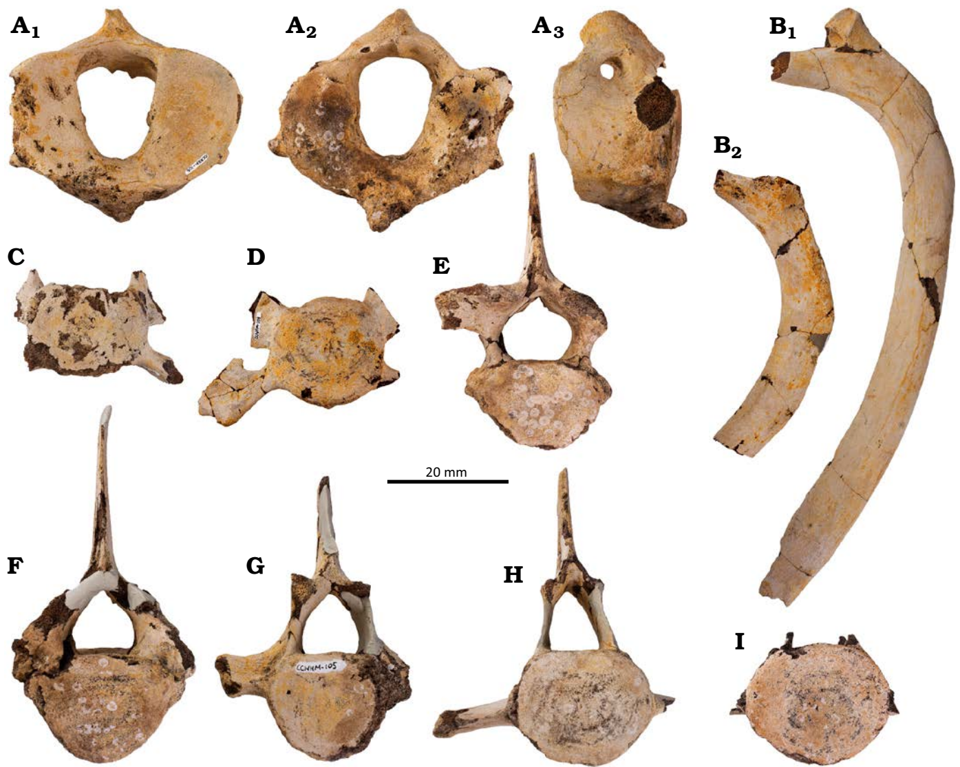
Fig. 4. Postcranial elements of the stem odontocete Ankylorhiza serratidens sp. nov. (CCNHM 105) from lower Oligocene Ashley Formation of Charleston, South Carolina, USA. A. Atlas in anterior ( A 1 ), posterior ( A 2 ), and left lateral ( A 3 ) views. B. Anterior left ribs in anterior view ( B 1 , B 2 ). Third cervical vertebra ( C ), fourth or fifth cervical vertebra ( D ), sixth or seventh thoracic vertebra ( E ), eighth thoracic vertebra ( F ), ninth thoracic vertebra ( G ), eleventh thoracic vertebra ( H ), and lumbar vertebra ( I ) in anterior view.
