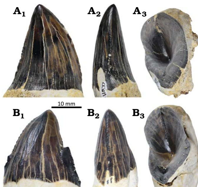
Fig. 3. Serrated postcanine teeth of the stem odontocete Ankylorhiza serratidens sp. nov. (CCNHM 105) from lower Oligocene Ashley Formation of Charleston, South Carolina, USA. A. Left pc3 crown in lingual (A 1 ), distal (A 2 ), and apical (A 3 ) views. B. Left pc5 crown in labial (B 1 ), mesial (B 2 ), and apical (B 3 ) views.
