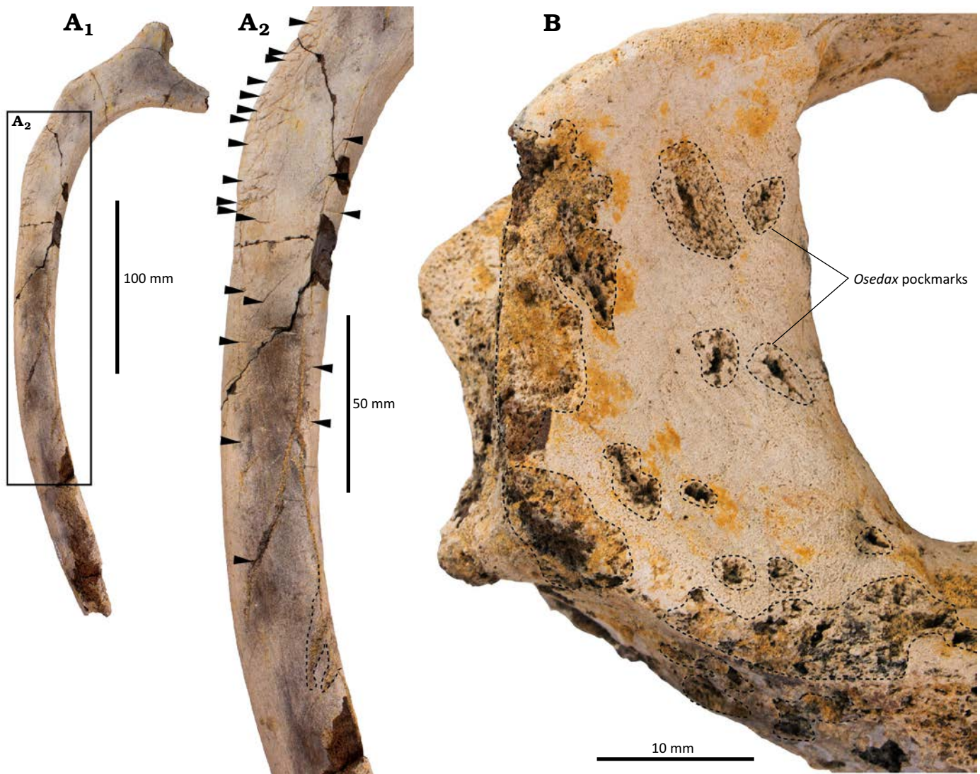
Fig. 5. Bone modifications in the stem odontocete Ankylorhiza serratidens sp. nov. (CCNHM 105) from lower Oligocene Ashley Formation of Charleston, South Carolina, USA. A. Left first rib in posterior view ( A_1 ), posterior face of rib ( A_2 ), showing location of traces attributed to shark feeding including linear bite marks (triangles) and shallow parallel grooves (dashed line). B. Right side of atlas in anterior view showing traces attributable to Osedax .
