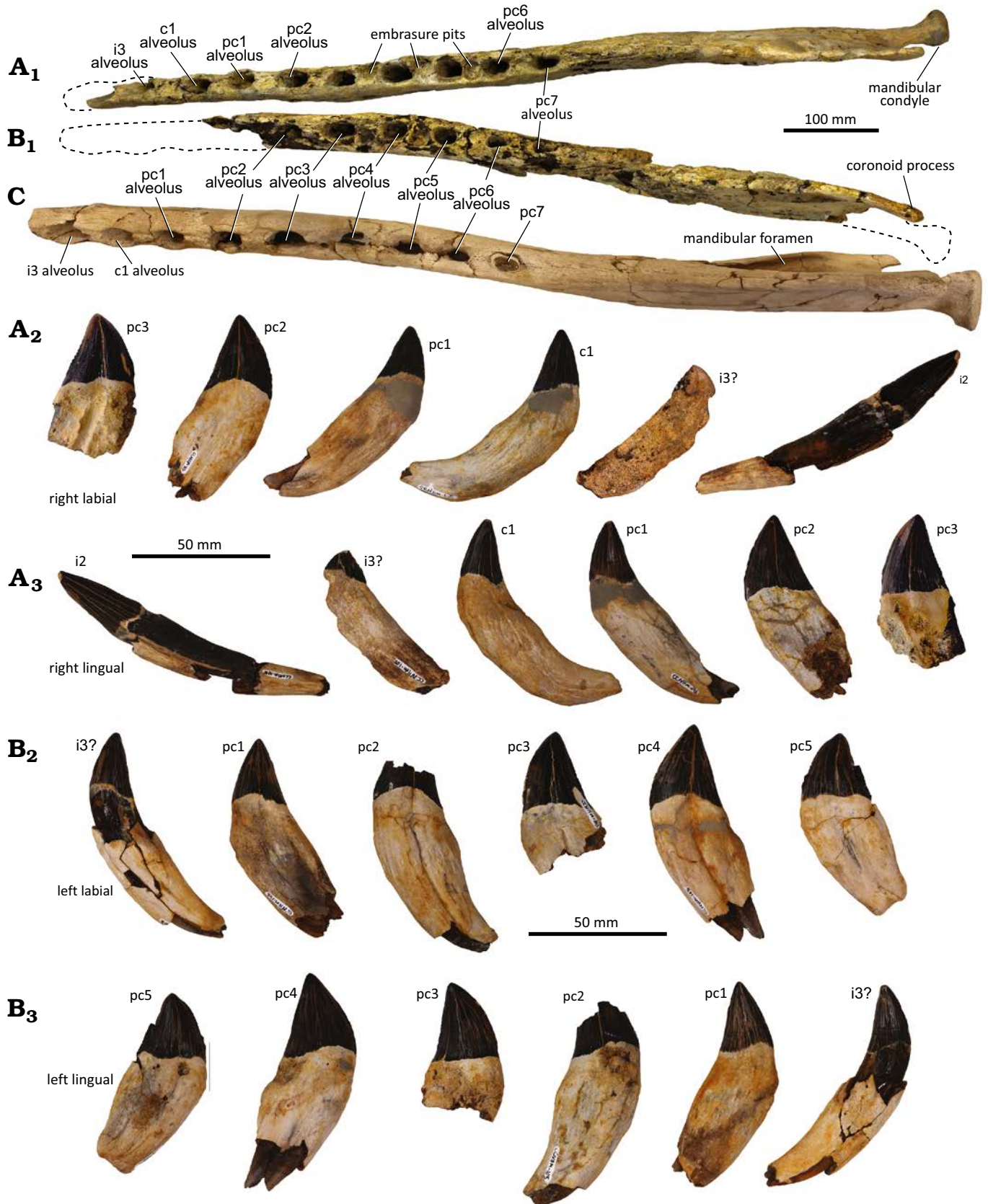
Fig. 2. Mandibles and teeth of the stem odontocete Ankylorhiza Boessenecker et al., 2020. A, B. Ankylorhiza serratidens sp. nov. (CCNHM 105) from lower Oligocene Ashley Formation of Charleston, South Carolina, USA. A. Right mandible in dorsal view (A 1 ), lower right anterior dentition in labial (A 2 ) and lingual (A 3 ) views. B. Left mandible in dorsal view (B 1 ), lower left anterior dentition in labial (B 2 ) and lingual (B 3 ) views. C. Ankylorhiza sp. (CCNHM 1075) from upper Oligocene Chandler Bridge Formation of Charleston, South Carolina, USA; left mandible in dorsal view.
