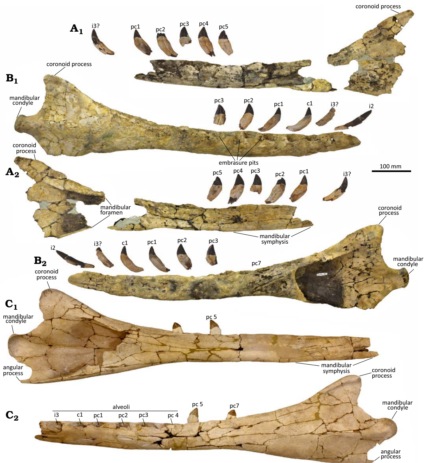
Fig. 1. Mandibles and teeth of the stem odontocete Ankylorhiza Boessenecker et al., 2020. A, B. Ankylorhiza serratidens sp. nov. (CCNHM 105) from lower Oligocene Ashley Formation of Charleston, South Carolina, USA. A. Left mandible and lower left dentition in lateral (A 1 ) and medial (A 2 ) views. B. Right mandible and lower right dentition in lateral (B 1 ) and medial (B 2 ) views. C. Ankylorhiza sp. (CCNHM 1075) from upper Oligocene Chandler Bridge Formation of Charleston, South Carolina, USA; left mandible in medial (C 1 ) and lateral (C 2 ) views.
