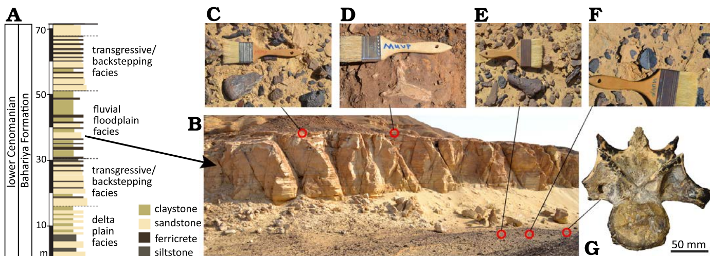
Fig. 2. Sedimentological context and fossil content of the Bahariya Formation in the Gebel El Dist region, Bahariya Oasis, Egypt. A. Lithological section of the Bahariya Formation at the Gebel El Dist locality, illustrating the first four facies associations of Catuneanu et al. (2006), including alternating sandstone, siltstone, claystone, and ferricrete horizons. B. Panoramic view of locality BOV16-10, which has yielded a diverse assemblage of vertebrate and plant fossils (C–G; specific recovery locations indicated by red circles). C. D. Osteichthyan ?cranial elements. E. Ornithocheiriform pterosaur wing phalanx (MUV 507) as it appeared upon discovery. F. Exceptionally preserved angiosperm leaves contained within ferruginous concretions. G. Previously described abelisaurid theropod dinosaur cervical vertebra (MUV 477; see Salem et al. 2022). All photos taken by MUV personnel.
